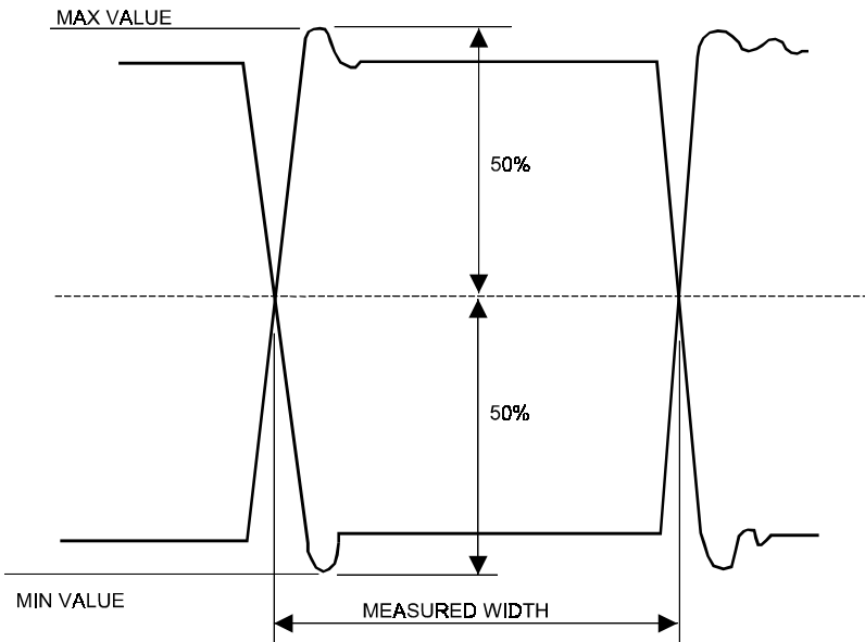
Figure 5-1, Positive/Negative Pulse
