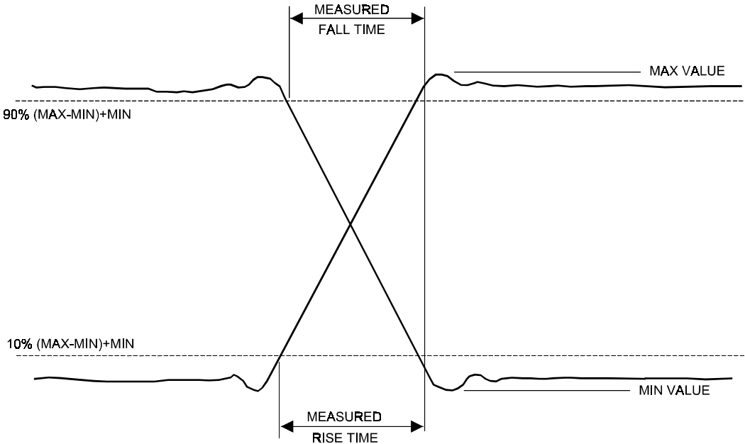
Figure 5-2, Rise/Fall Time
