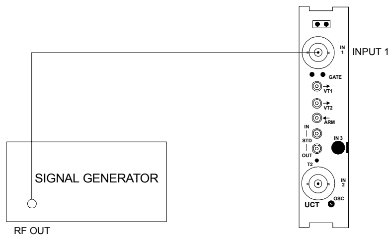
Figure 6-7, Input 1 Filter Check Configuration
